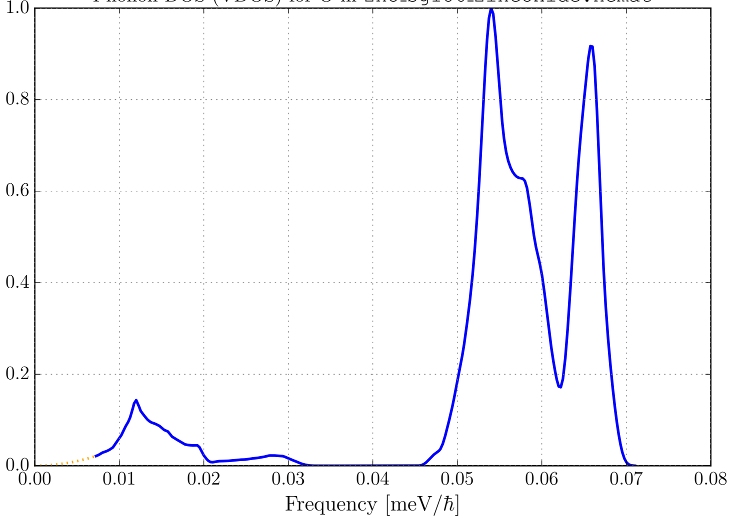
Phonon DOS (VDOS) for O in ZnO_sg186_ZincOxide.ncmat
