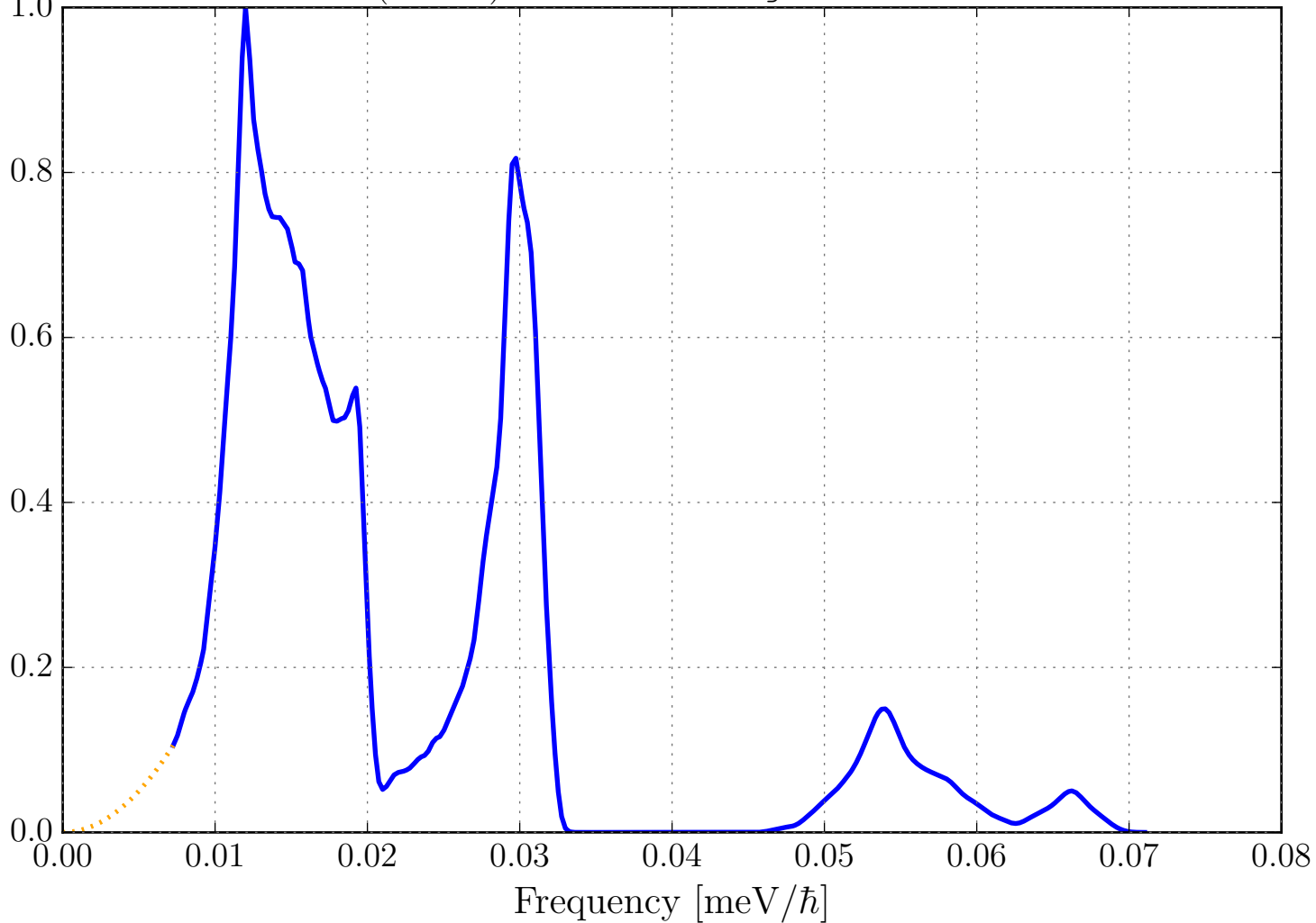
Phonon DOS (VDOS) for Zn in ZnO_sg186_ZincOxide.ncmat
