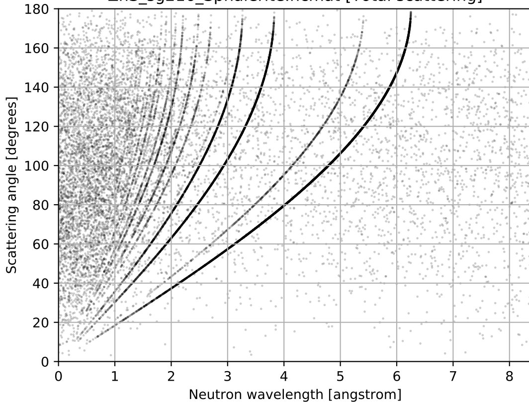
ZnS_sg216_Sphalerite.ncmat [Total scattering]
