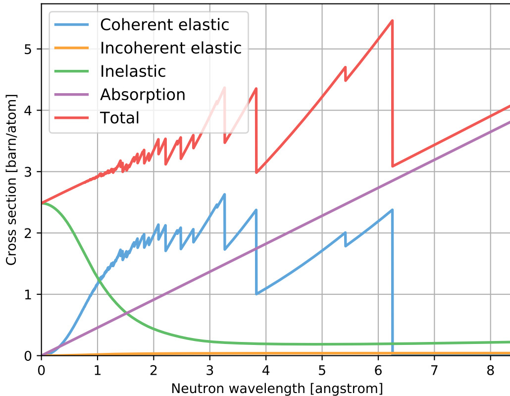
ZnS_sg216_Sphalerite.ncmat
