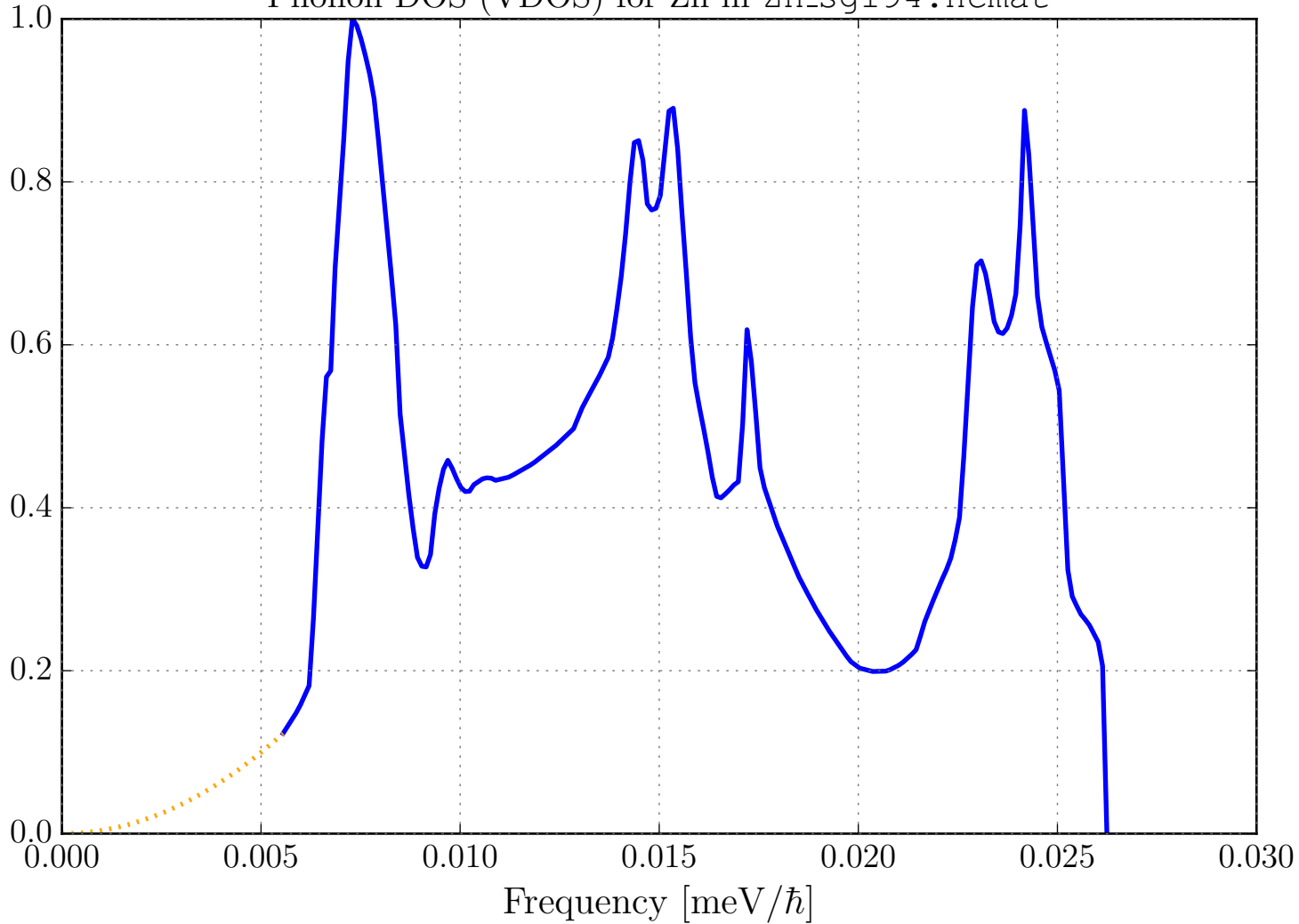
Phonon DOS (VDOS) for Zn in Zn_sg194.ncmat
