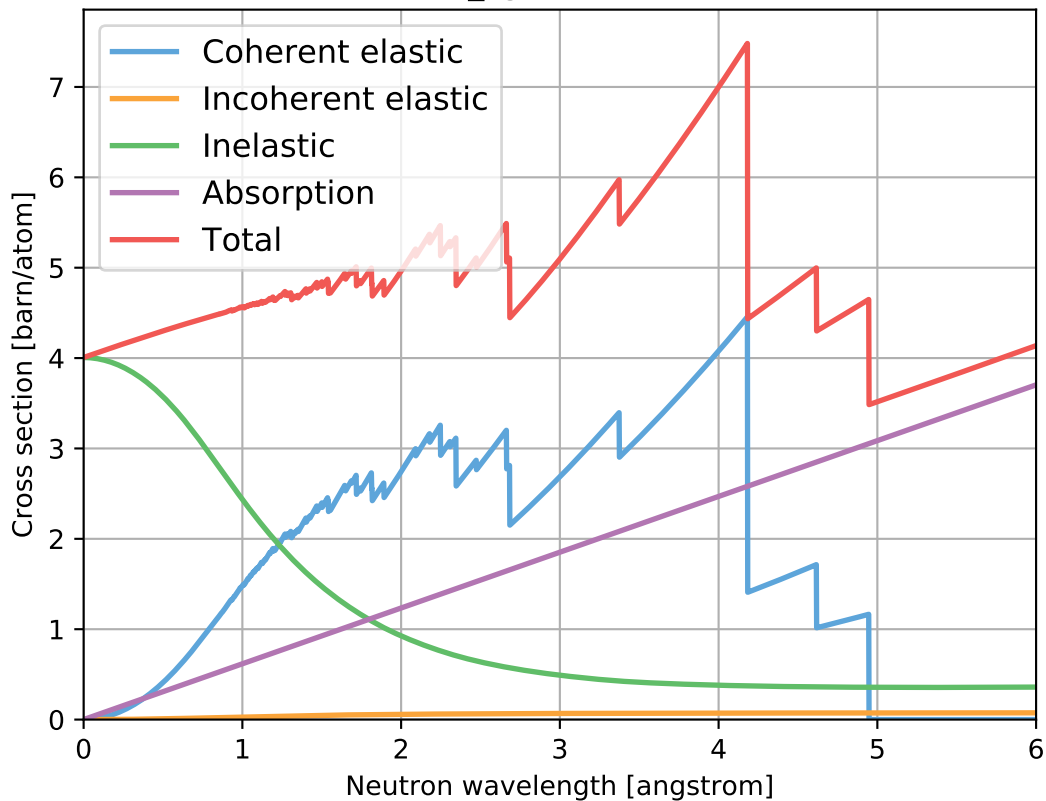
Zn_sg194.ncmat
