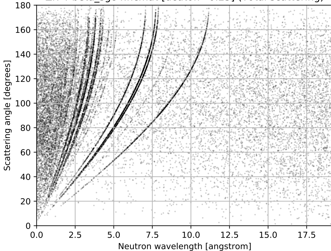
ZrF4-beta_sg84.ncmat [dcutoff=0.25] (Total scattering)
