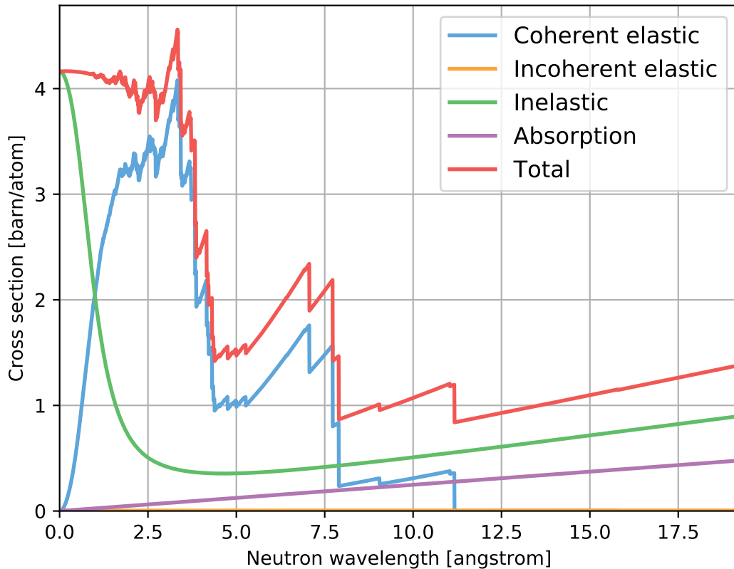
ZrF4-beta_sg84.ncmat [dcutoff=0.25]
