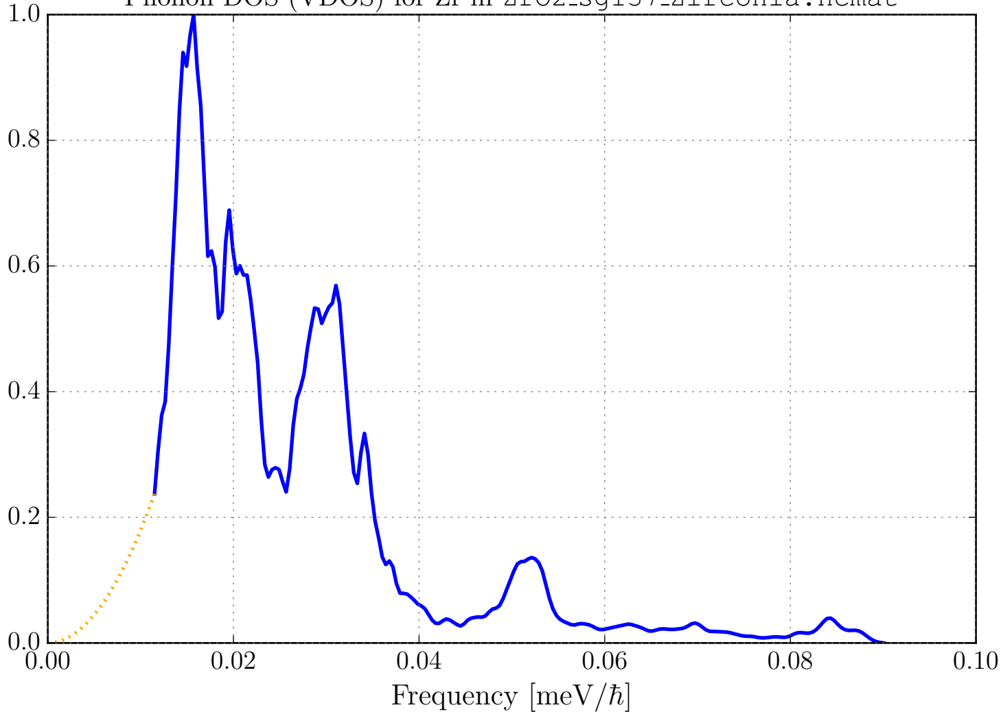
Phonon DOS (VDOS) for Zr in ZrO2_sg137_Zirconia.ncmat
