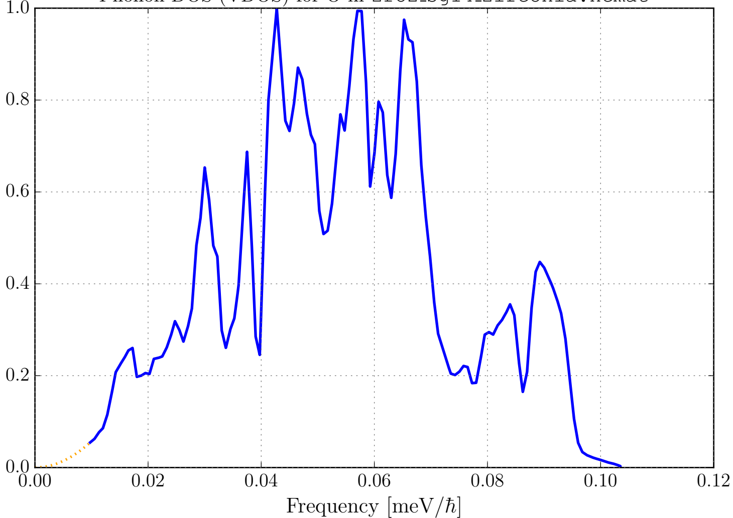
Phonon DOS (VDOS) for O in ZrO2_sg14_Zirconia.ncmat
