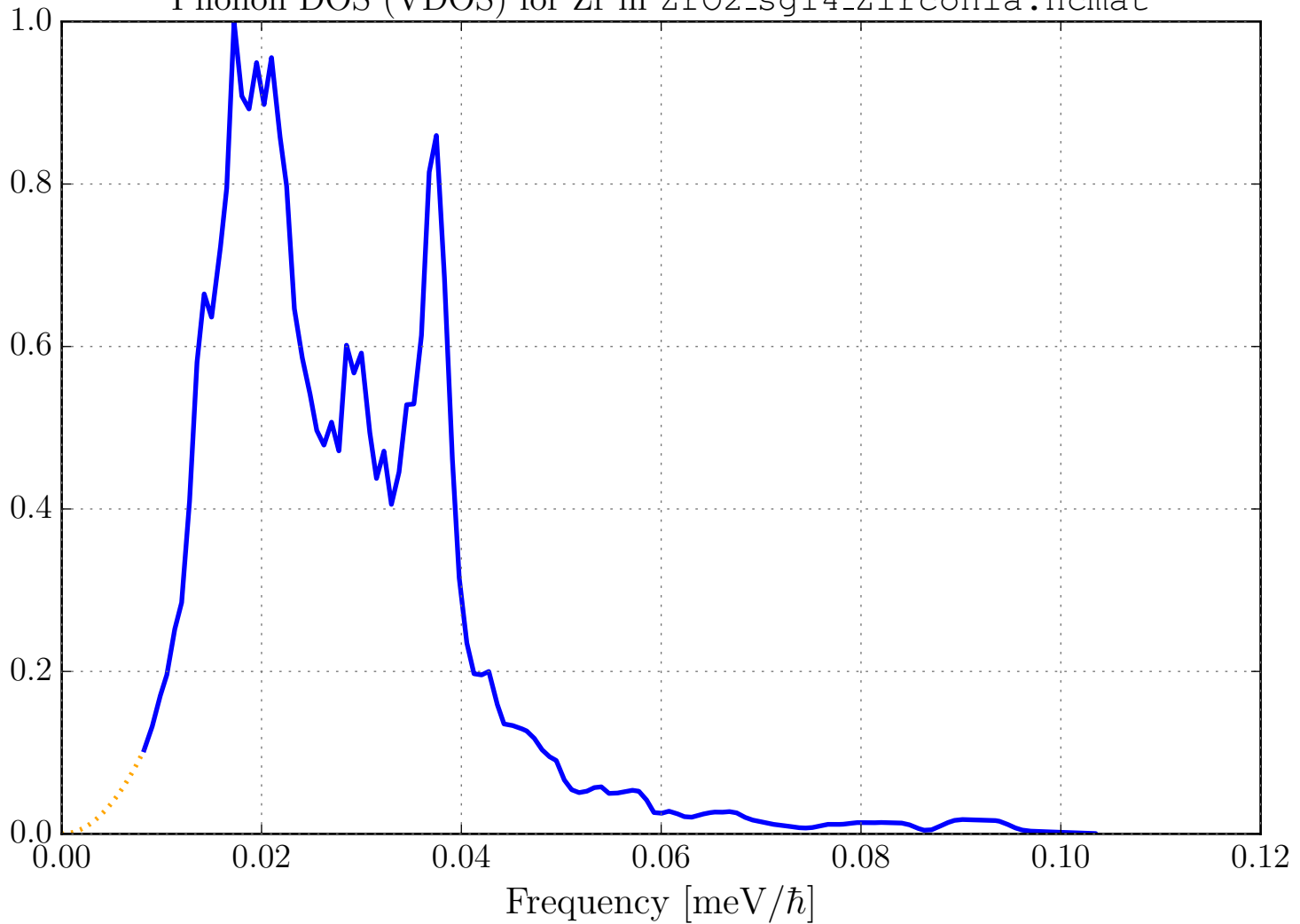
Phonon DOS (VDOS) for Zr in ZrO2_sg14_Zirconia.ncmat
