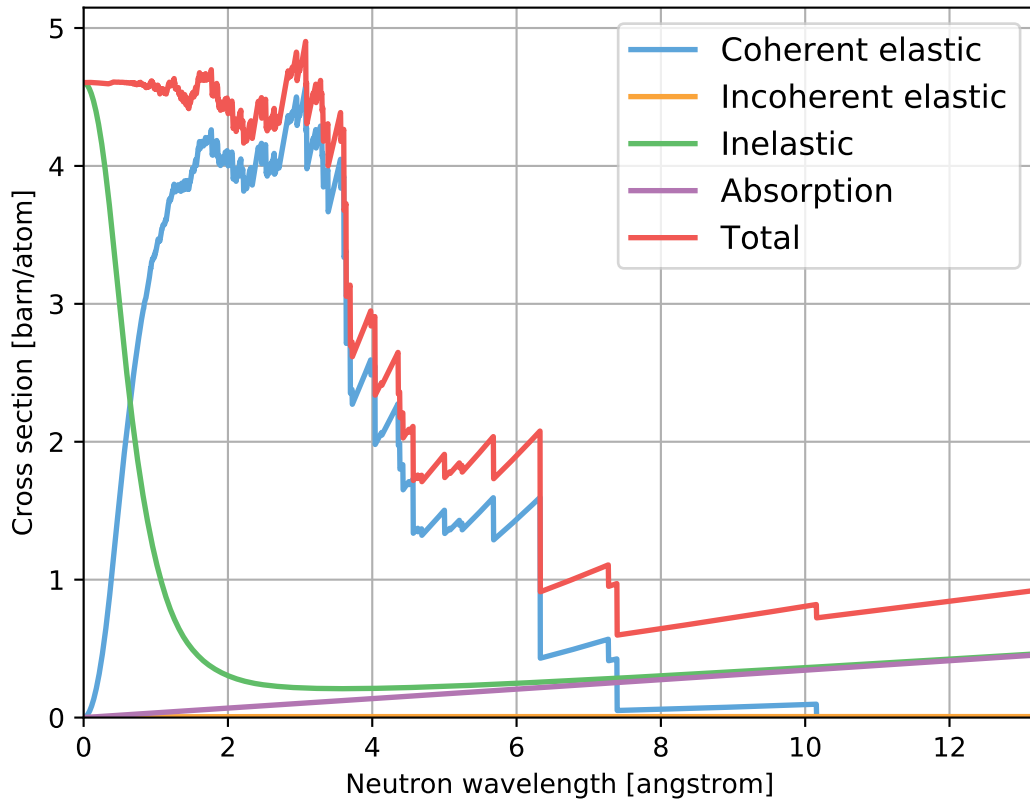
ZrO2_sg14_Zirconia.ncmat [dcutoff=0.2]
