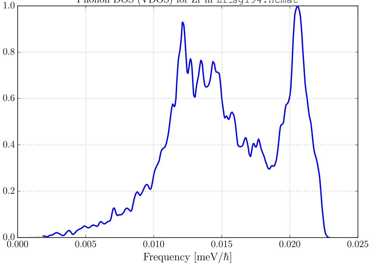
Phonon DOS (VDOS) for Zr in Zr_sg194.ncmat
