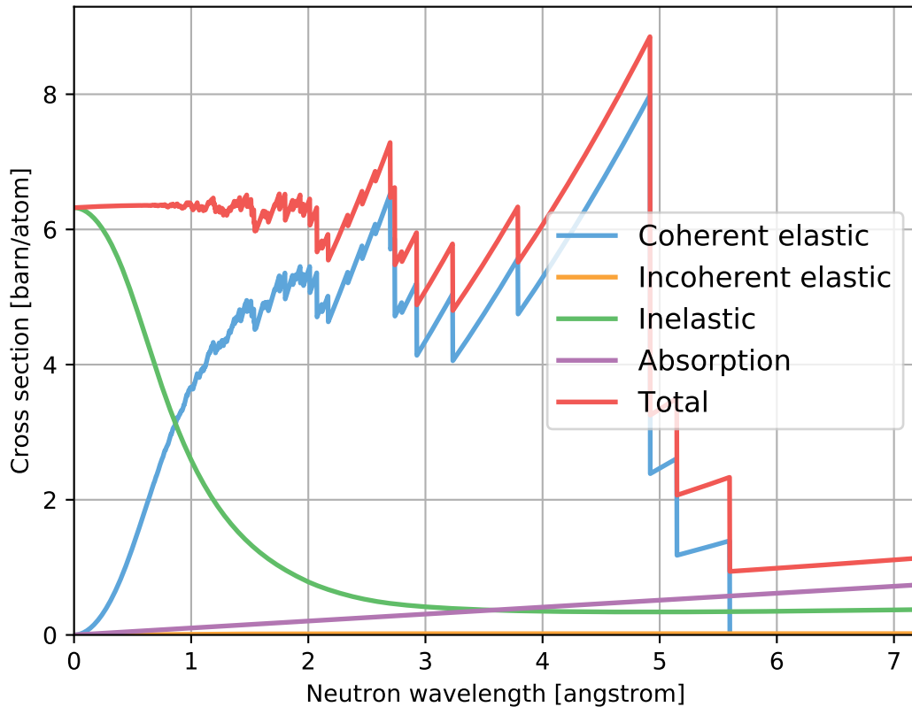
Zr_sg194.ncmat
