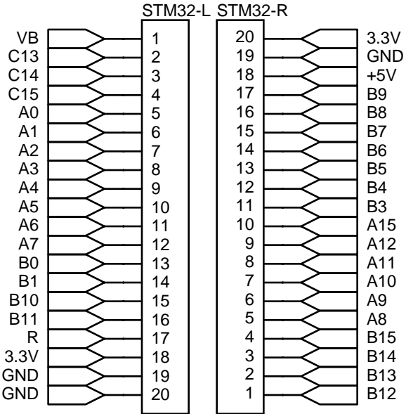
STM32F103C8T6
