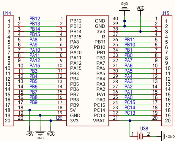
STM32F103C8T6
