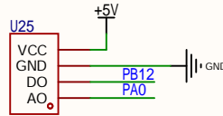
MQ2
