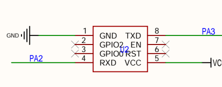
ESP8266-01s模块
