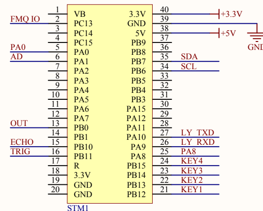
STM32F103C8T6单片机芯片
