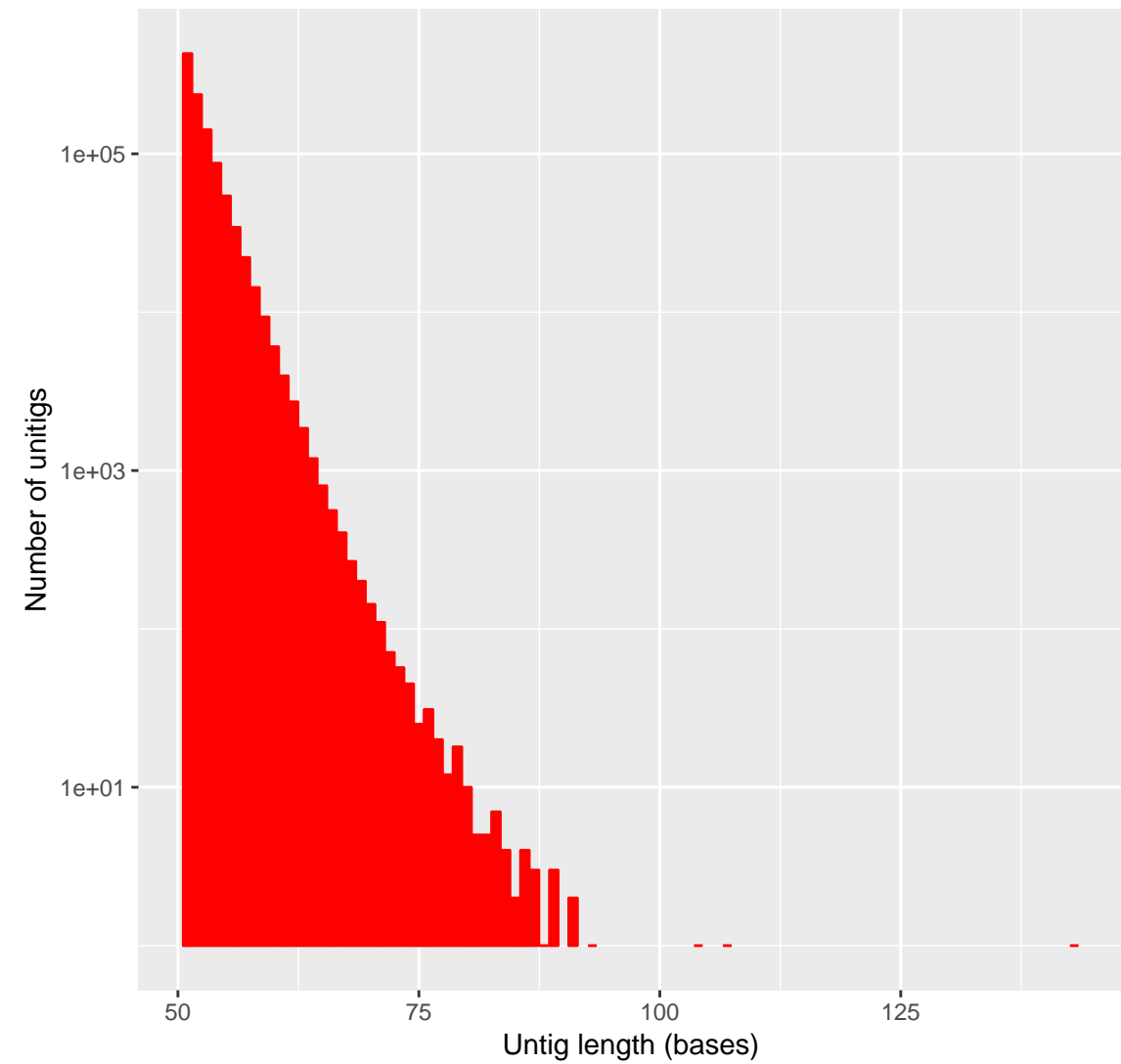
Clean Unitig Length
