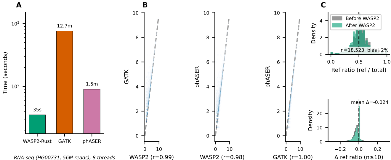
Figure 2: Allele Counting - RNA-seq
