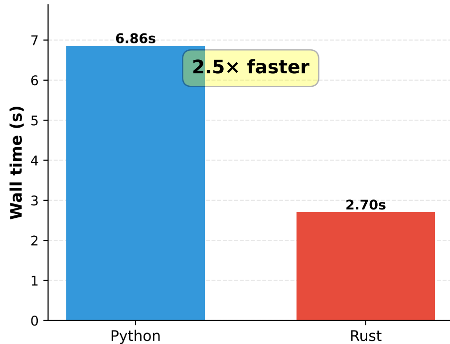
A. Allele Counting (111K SNPs, chr10)
