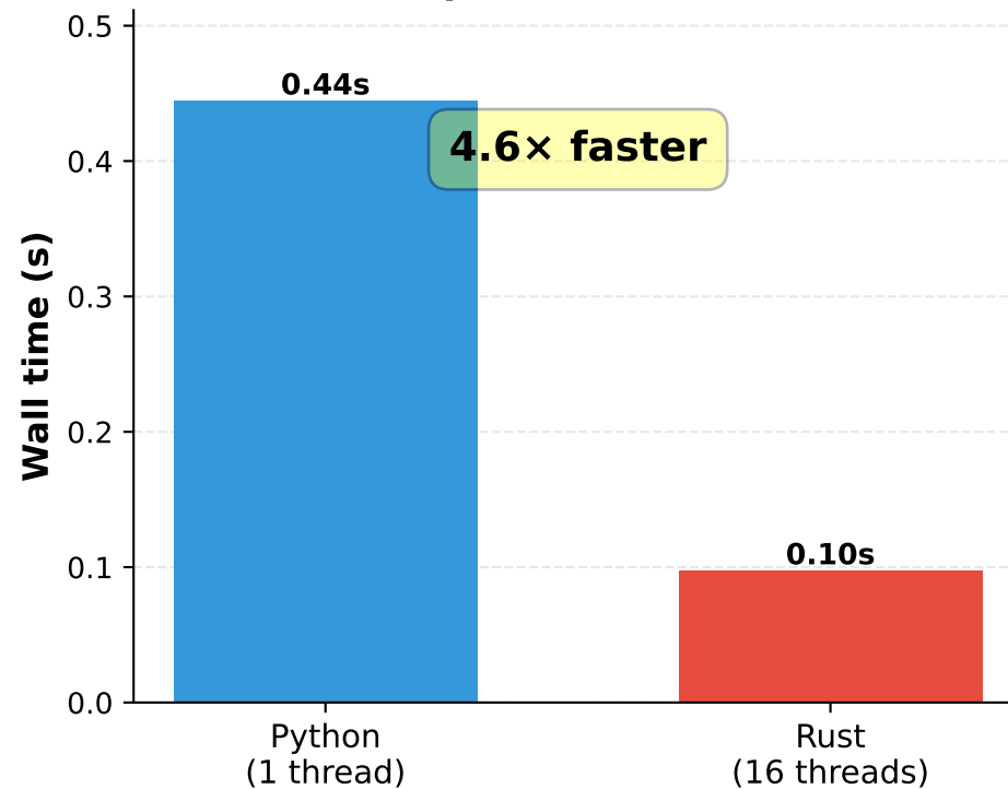
B. Mapping Filter (20K pairs, 16 threads)
