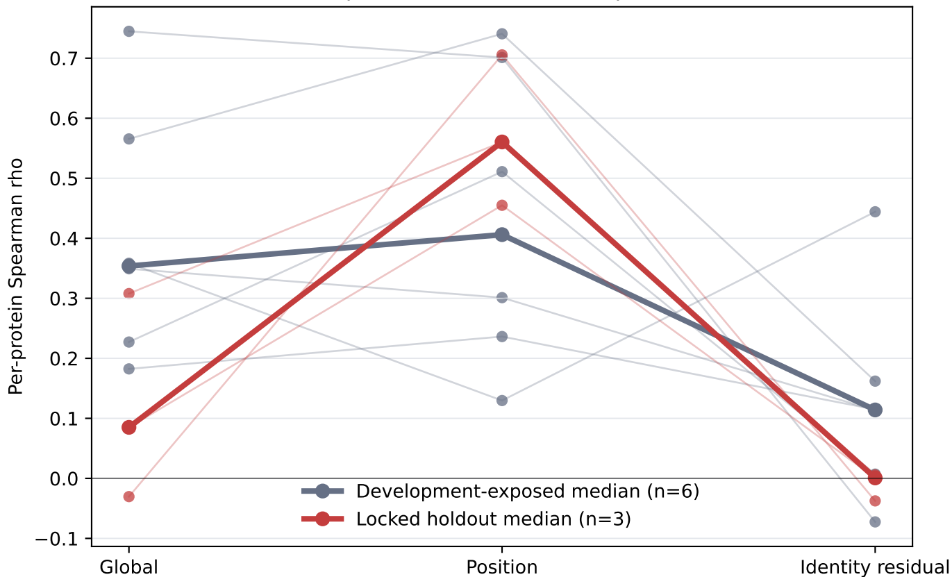
DeepPBS local-effect decomposition
