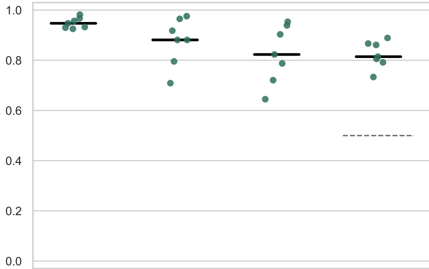
Canonical Watson-Crick mutations (primary)
