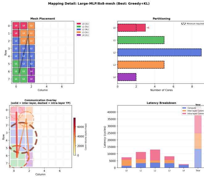
Fig. 4. Greedy+KL mapping for Large-MLP/8 \times 8 (42.7 \mu s): mesh placement, partition, communication overlay, and per-layer latency.
