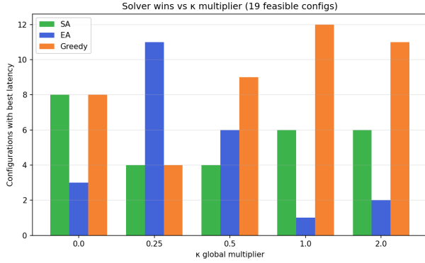
Fig. 3. Solver wins as a function of the \kappa multiplier.
