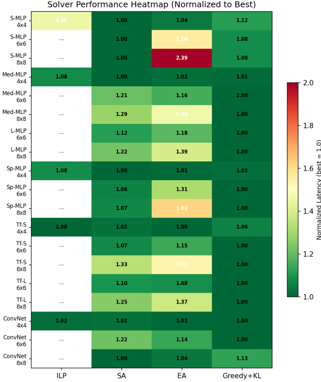
Fig. 1. Normalized latency (best joint optimizer per config = 1.0).
