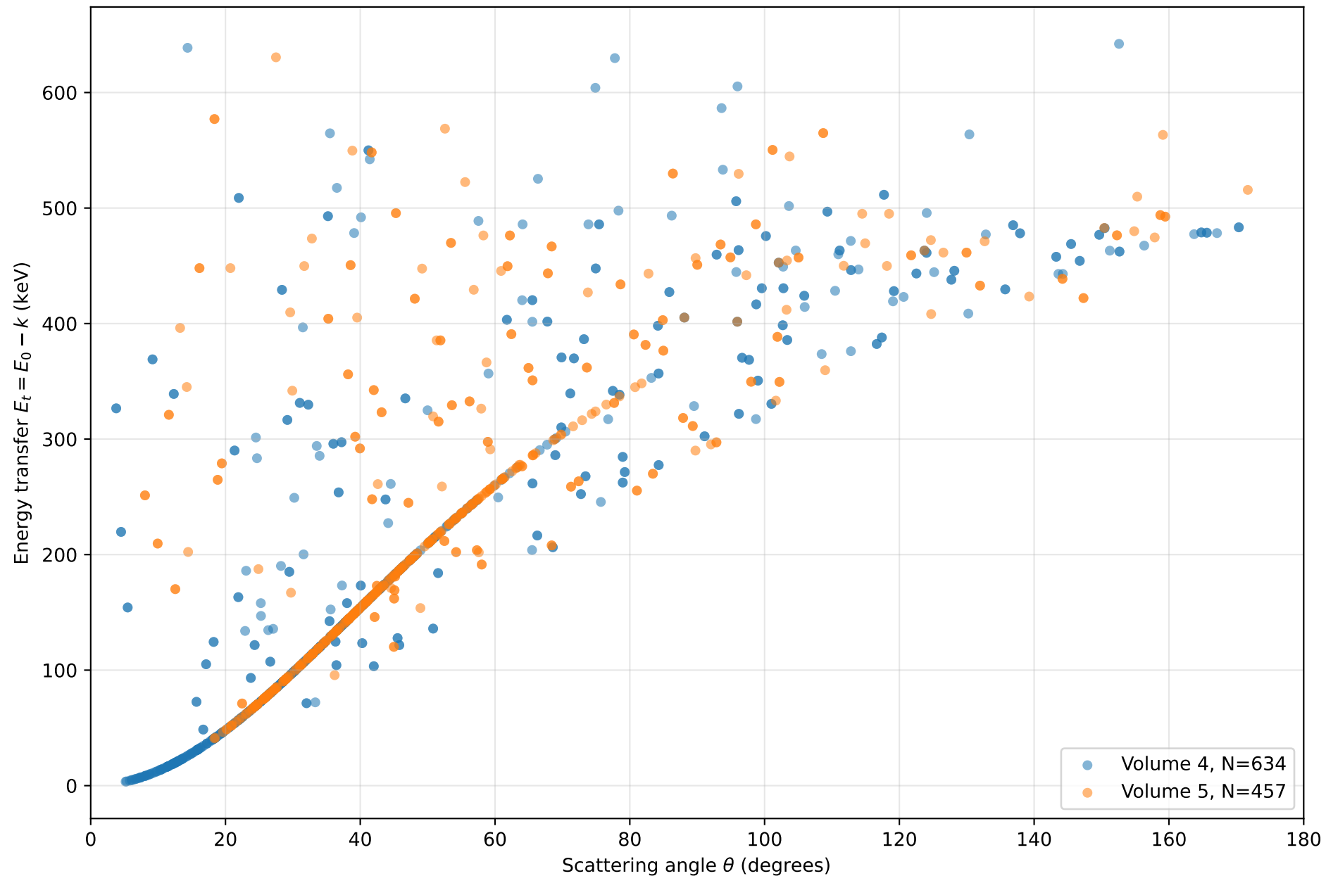
Energy transfer E_t versus angle: detector volumes 4 and 5
