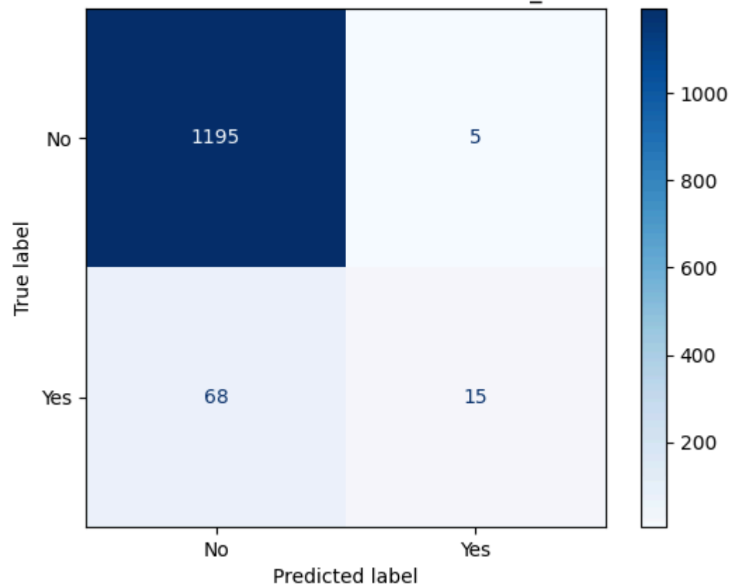
Confusion Matrix for Class: connected_crack
