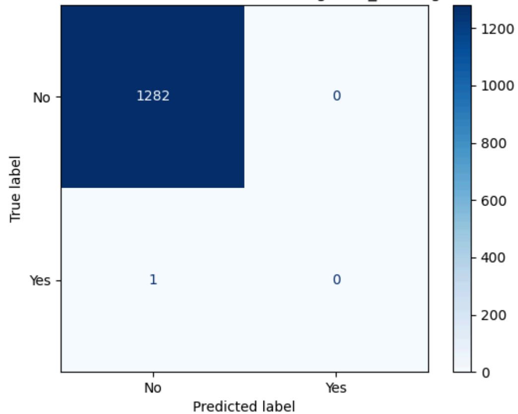
Confusion Matrix for Class: corrugation_shoving
