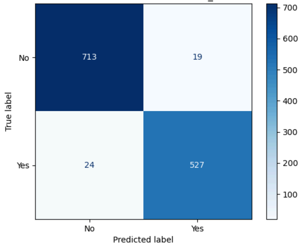
Confusion Matrix for Class: sidewalk_shoulder
