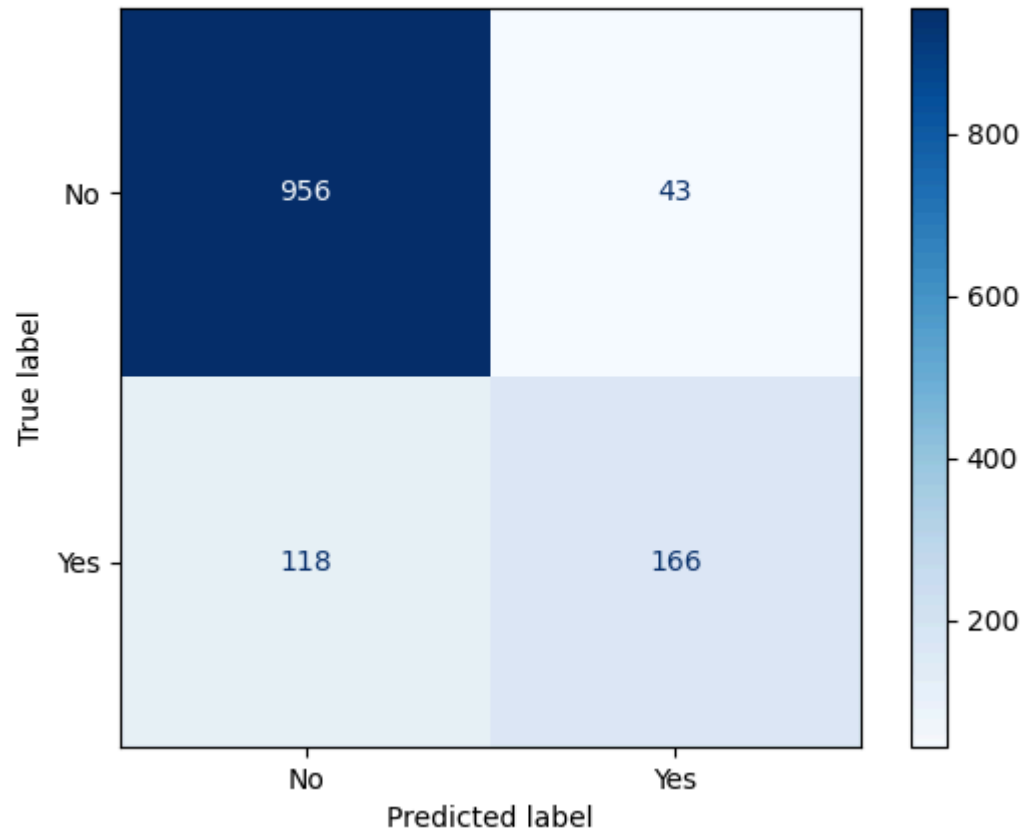
Confusion Matrix for Class: pothole
