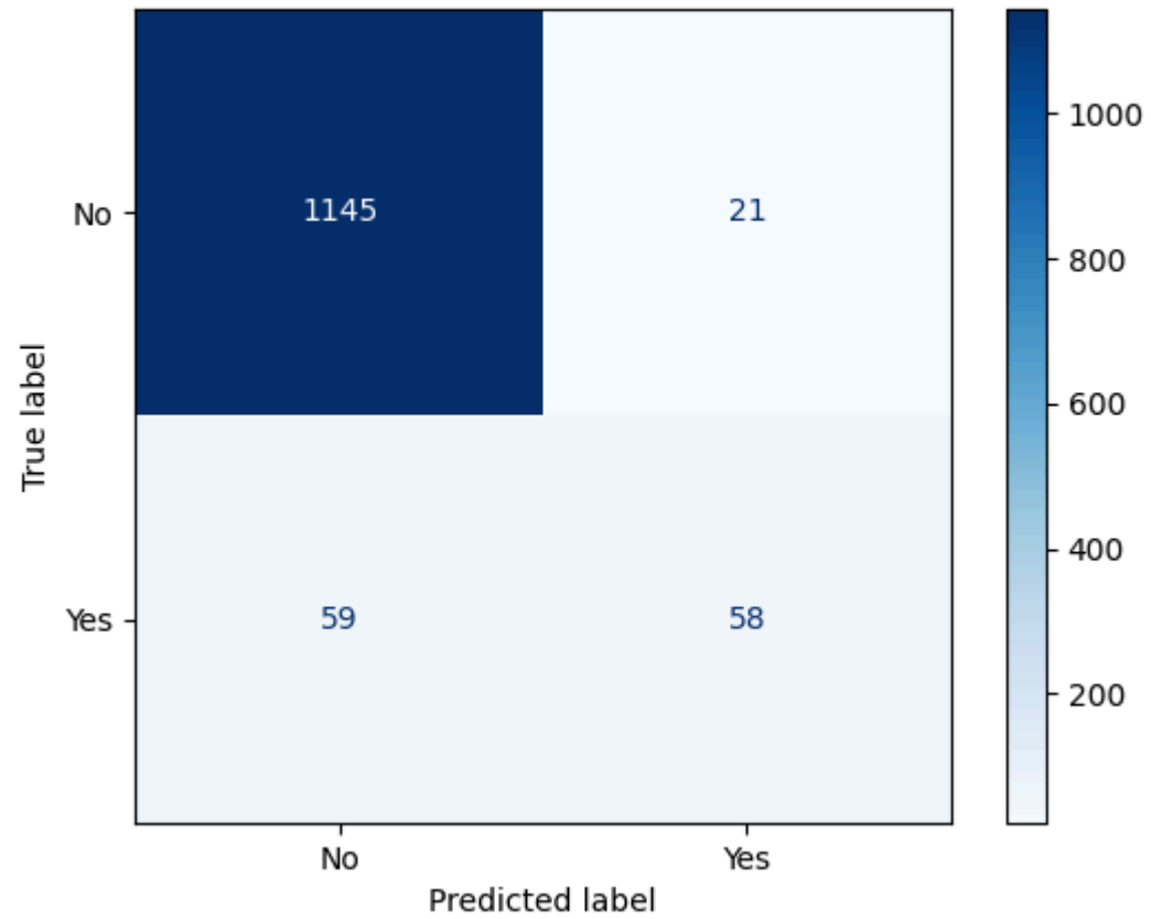
Confusion Matrix for Class: bleeding
