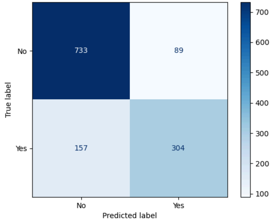
Confusion Matrix for Class: patch
