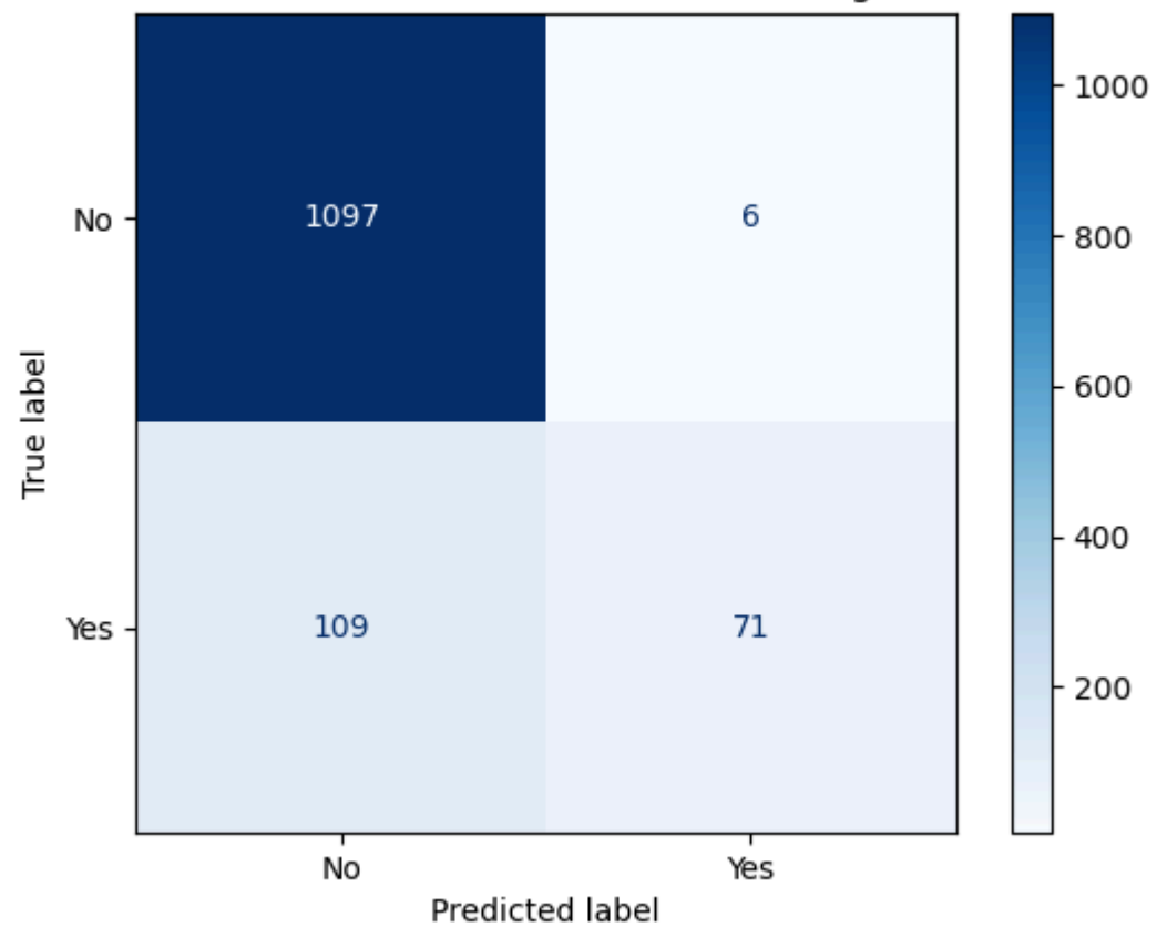
Confusion Matrix for Class: raveling
