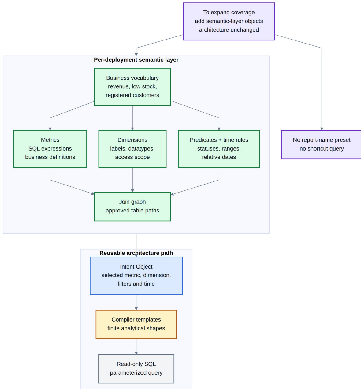
Figure 3: Semantic layer modularity - composable blocks vs. free-form SQL generation
