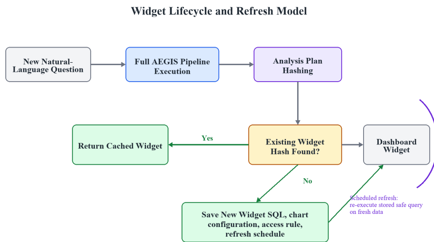
Fig. 4 Widget lifecycle for reusable natural-language analytics.
