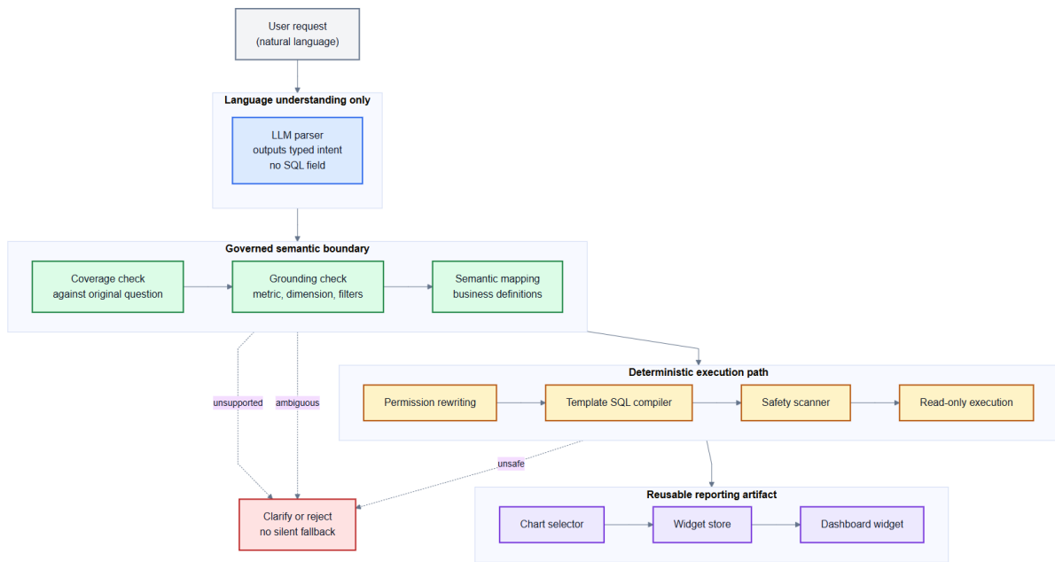
Figure 2: AEGIS architecture pipeline (User Request to Dashboard Widget)
