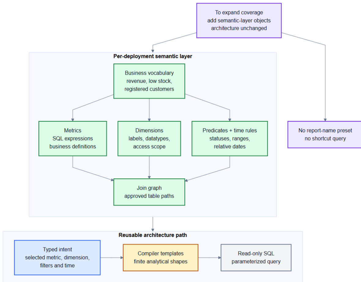
Figure 3: Semantic layer modularity - composable blocks vs. free-form SQL generation
