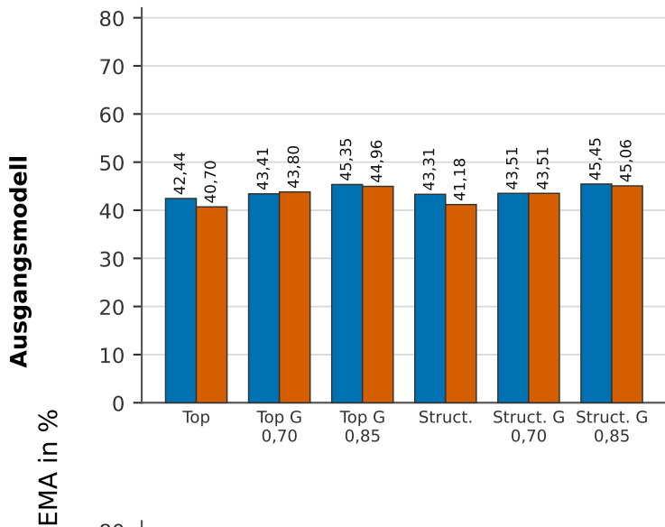
Qwen 3.5 2B
