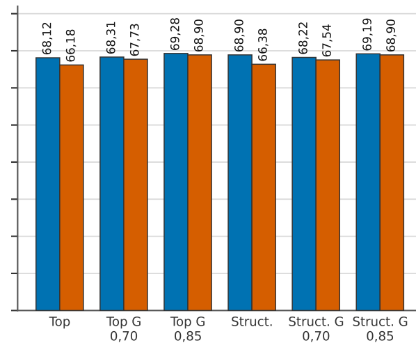
Qwen 3.5 9B
