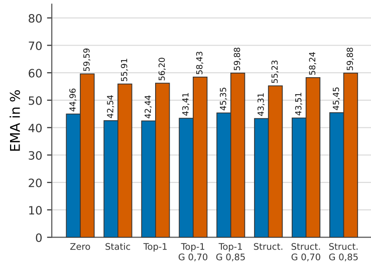
(a) Qwen 3.5 2B
