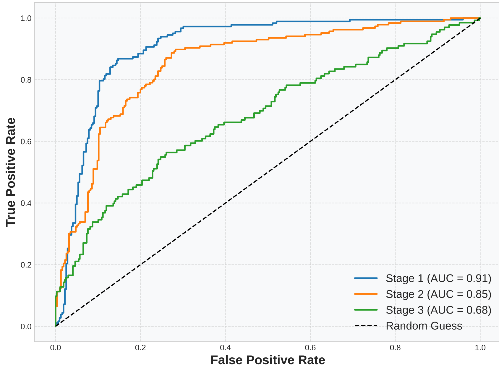
ROC Curves on Validation Set
