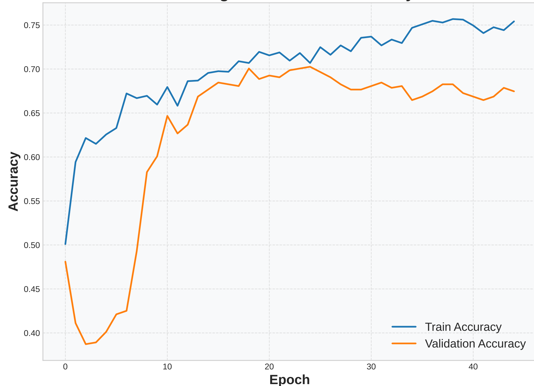
Training vs Validation Accuracy
