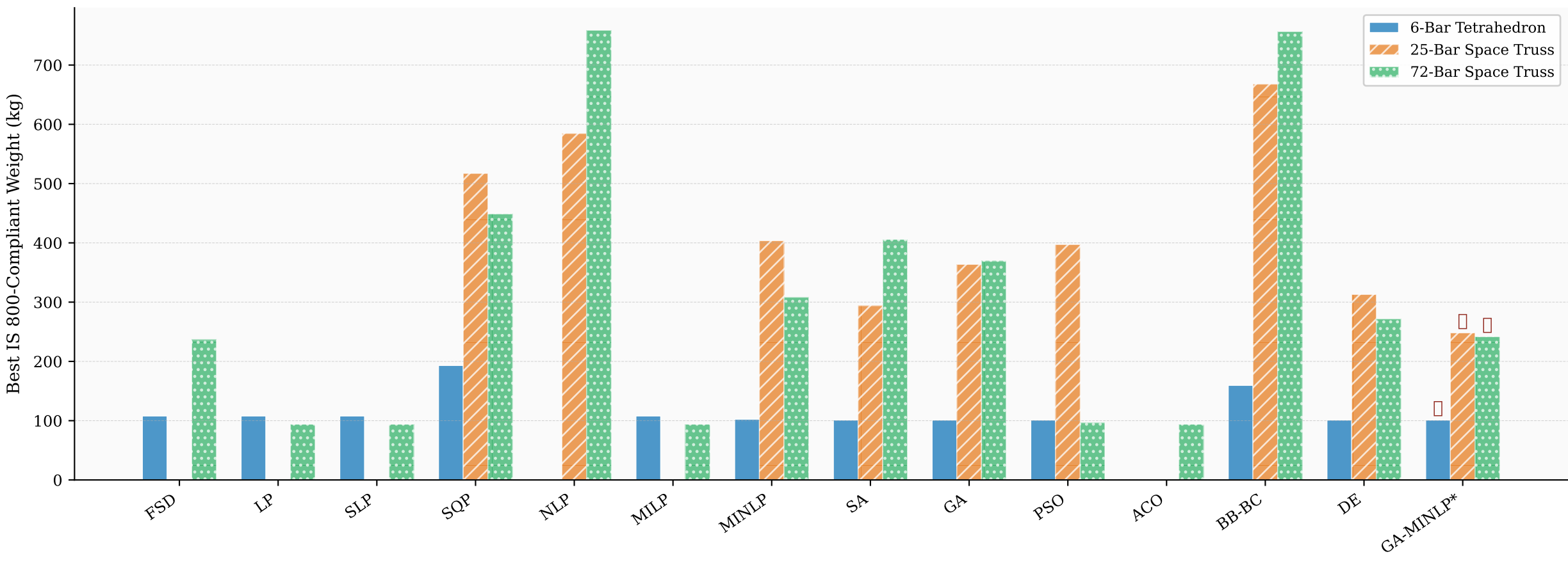
All-Method Weight Comparison — Three Benchmark Trusses
