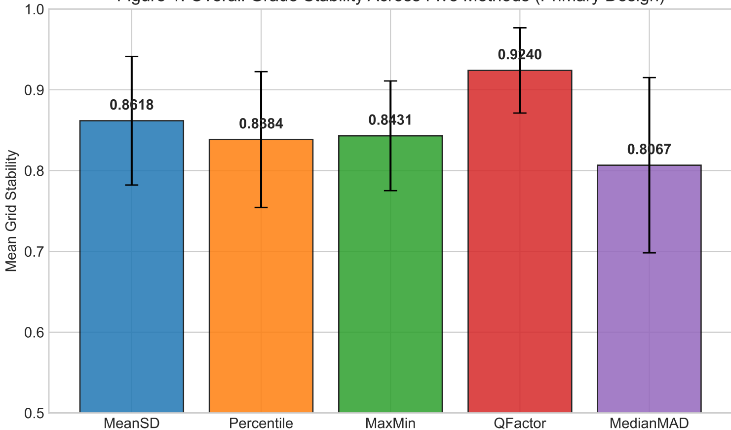
Figure 1: Overall Grade Stability Across Five Methods (Primary Design)
