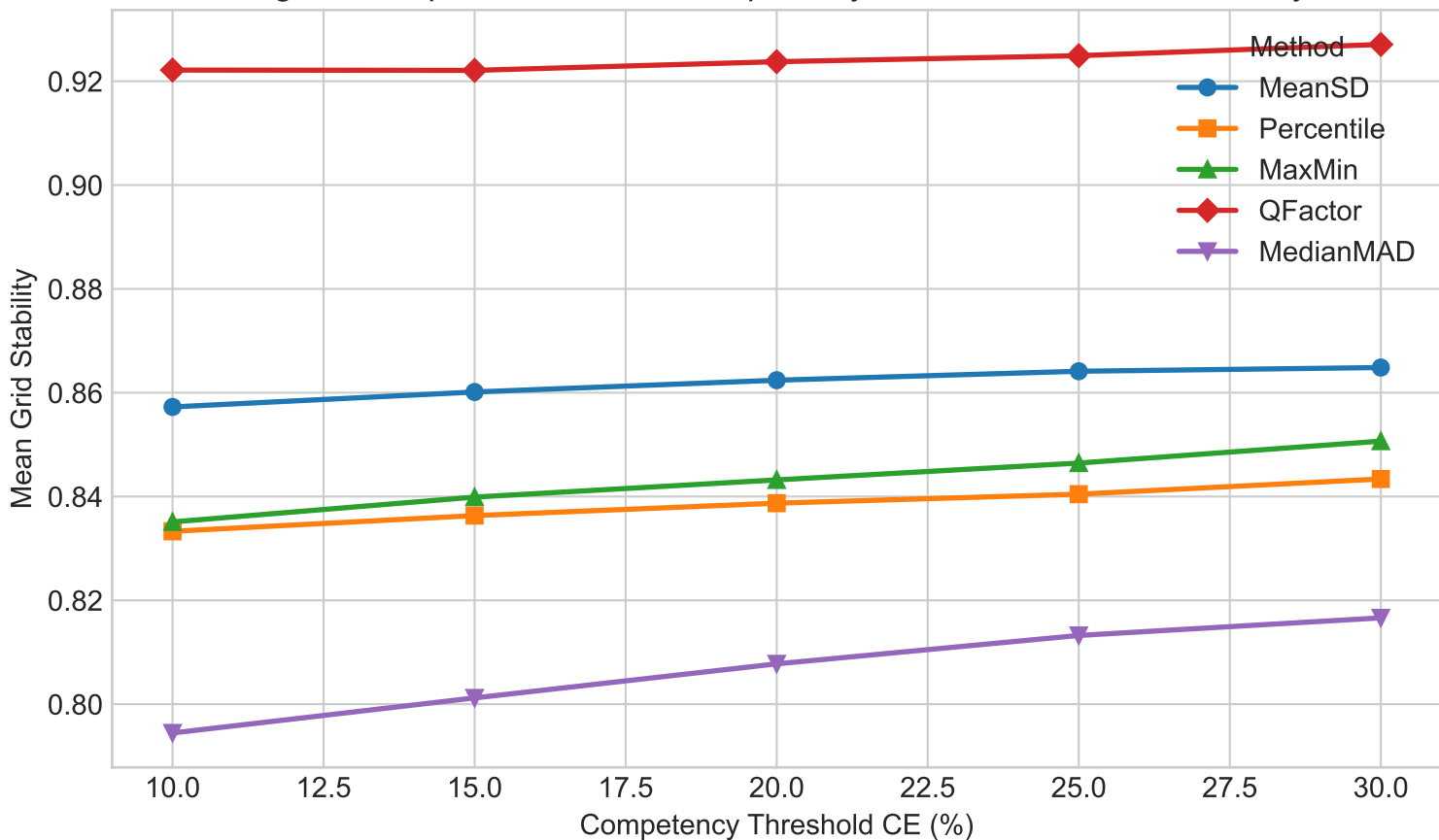
Figure 4: Impact of External Competency Threshold on Grade Stability
