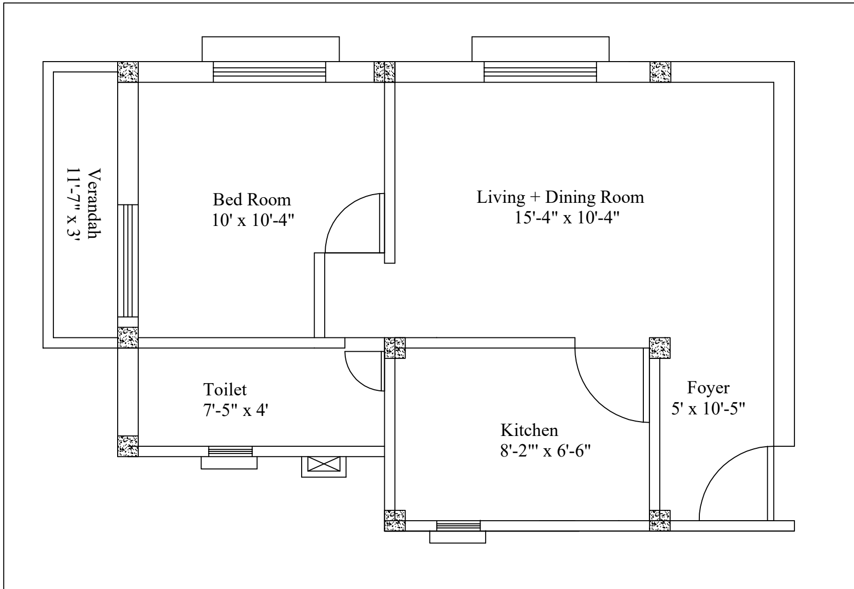
Fig: Residential Unit Plan-2 Scale: Not to scale
