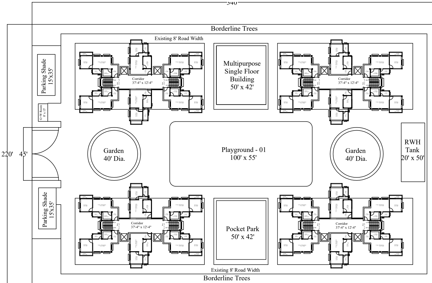
Fig.: Masterplan Scale: Not to scale
