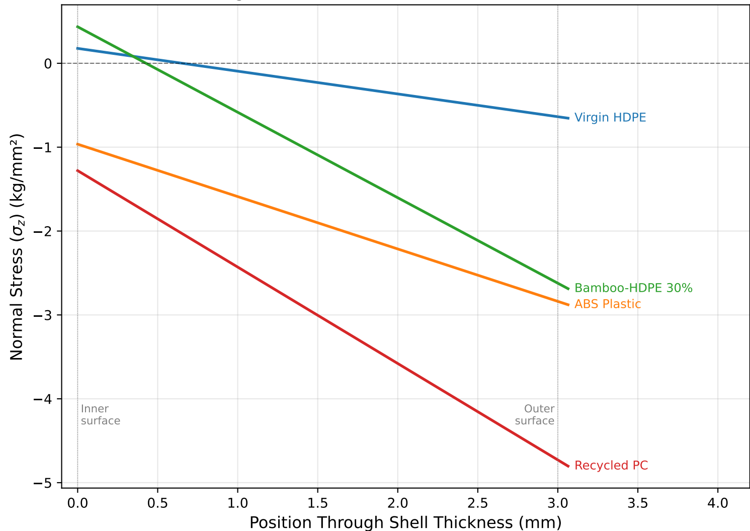
Through-Thickness Normal Stress at Helmet Crown
