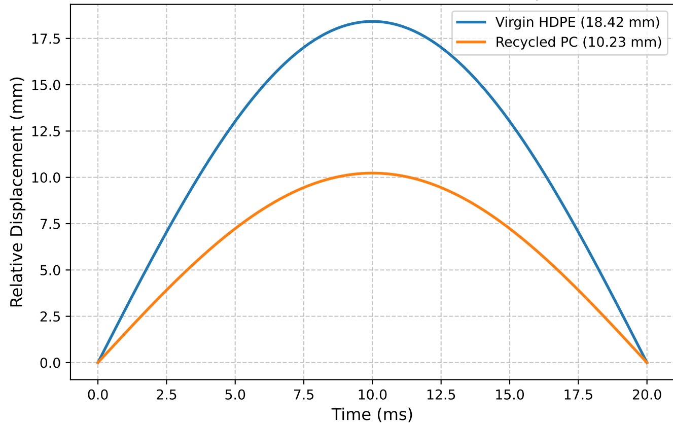
Phase 5: Kinematic Crush Depth (Relative Displacement)
