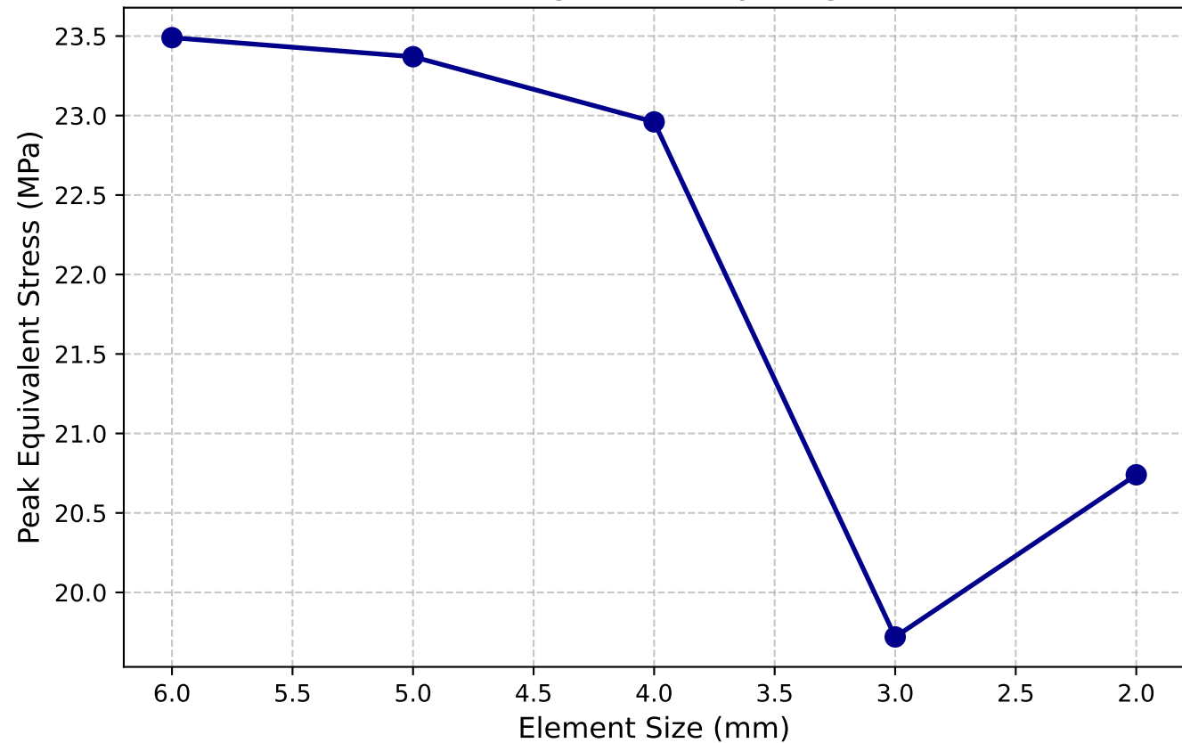
Mesh Convergence Study: Virgin HDPE
