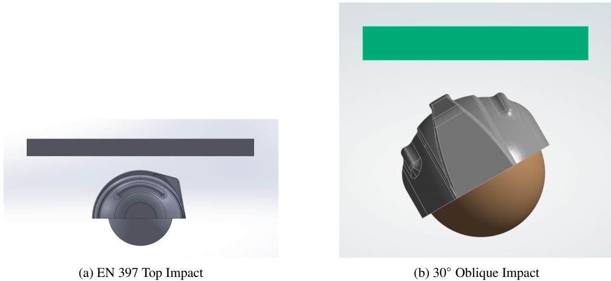
Figure 3.1: Numerical assembly and impact configurations. The Galilean upward velocity shift is applied to the headform-helmet assembly against a stationary rigid boundary.
