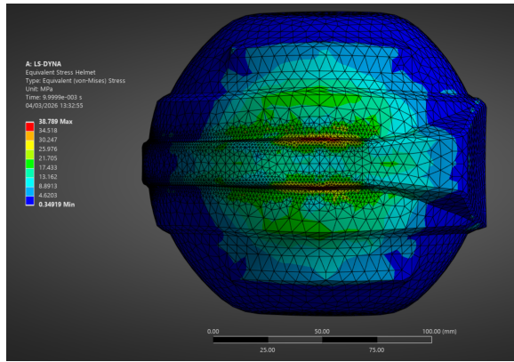
(a) Virgin HDPE
