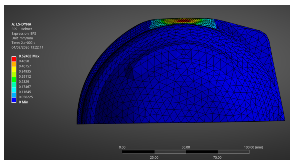
(a) Virgin HDPE (Localized strain)
