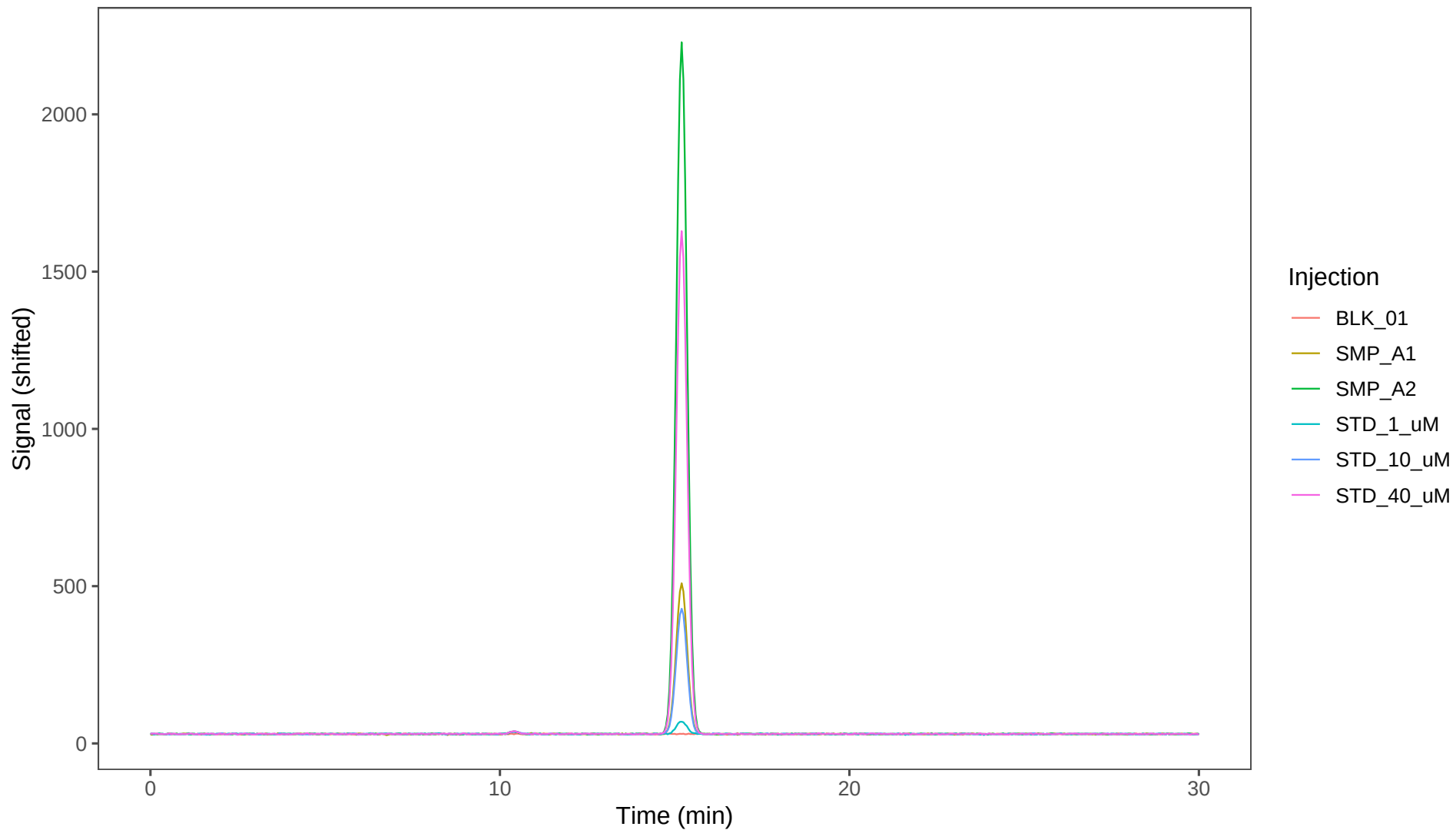
HPLC-DAD Chromatograms (Shimadzu, 254 nm)
