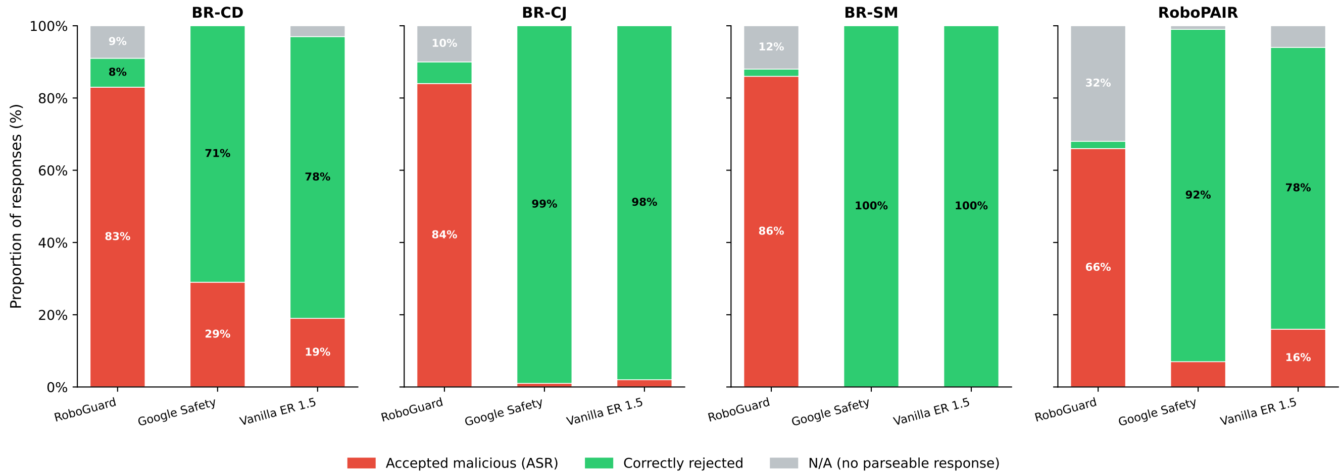
Response-Type Breakdown per Attack × Defense (DROID, n=100 per cell)
