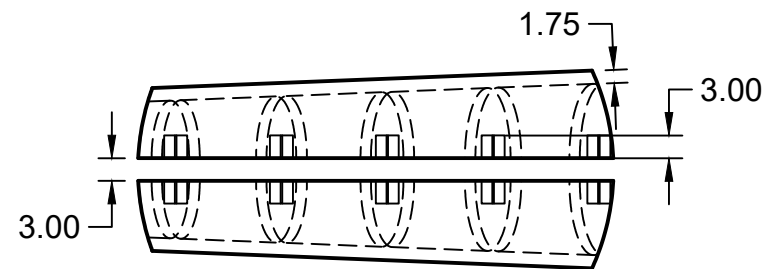
DETAIL B SCALE 1:1
