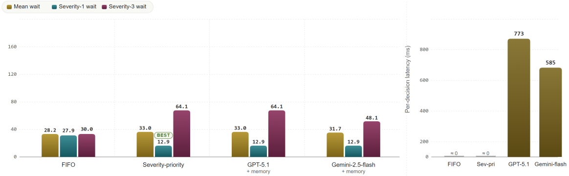
Figure 8: Per-policy wait times (left) and wall-time cost per admission decision (right).
