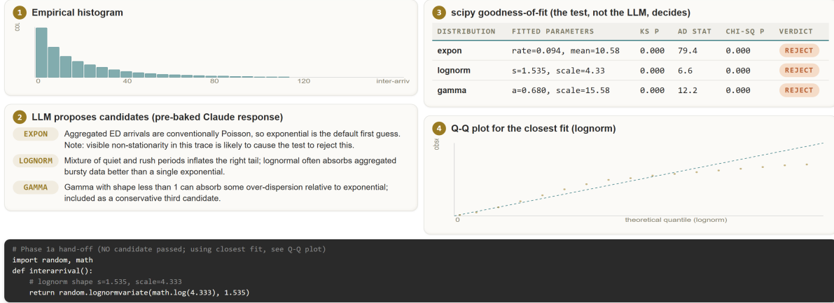
Figure 6: Input modelling on a deliberately bursty ED arrival trace. The LLM proposes three candidate distributions with one-line rationales; scipy.stats fits each and runs KS, AD, and chi-square goodness-of-fit. All three candidates are rejected at the 5% level. The Q-Q plot shows systematic deviation in the upper tail, and the verdict (written by the LLM after reading the test output) recommends refitting per hour-of-day.
