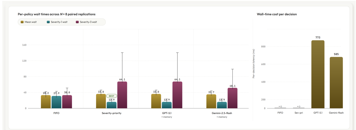
Figure 9: Results of Table 1 as a bar chart, rendered directly from summary.json . Left: per-policy wait times with \pm 1 std error bars. Right: wall-time cost per admission decision. GPT-5.1 with memory matches severity-priority bar-for-bar; Gemini-2.5-flash with memory drops Sev-3 wait from 64.1 to 48.1 minutes while keeping Sev-1 wait constant.
