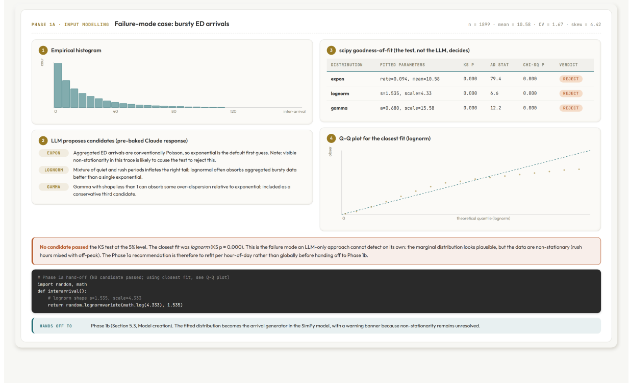
Figure 7: Input modelling on a deliberately bursty ED arrival trace. The LLM proposes three candidate distributions with one-line rationales; scipy.stats fits each and runs KS, AD, and chi-square goodness-of-fit. All three candidates are rejected at the 5% level. The Q-Q plot shows systematic deviation in the upper tail, and the verdict (written by the LLM after reading the test output) recommends refitting per hour-of-day.
