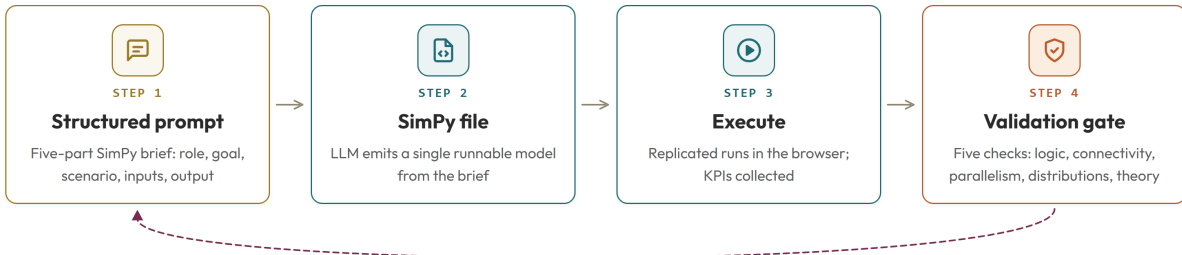
Figure 7: Vibe-coding loop with a five-check validation gate.
