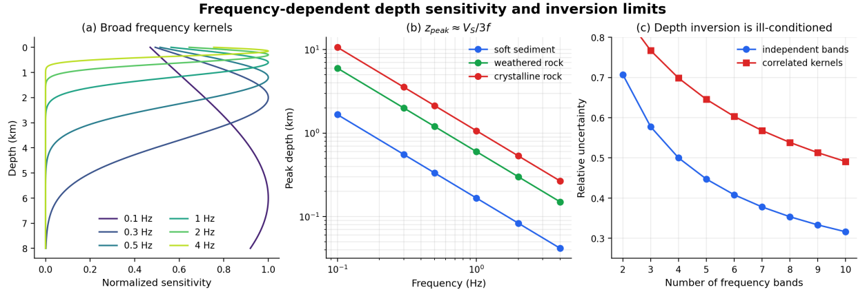
Figure 6: Frequency-dependent depth sensitivity and inversion limits. (a) Schematic Rayleigh/Love sensitivity kernels showing broad, overlapping depth sensitivity for representative frequency bands. (b) Peak sensitivity depth z_{peak} \approx V_S/(3f) for soft sediment, weathered rock, and crystalline rock. (c) Relative uncertainty reduction for independent versus correlated frequency bands.
