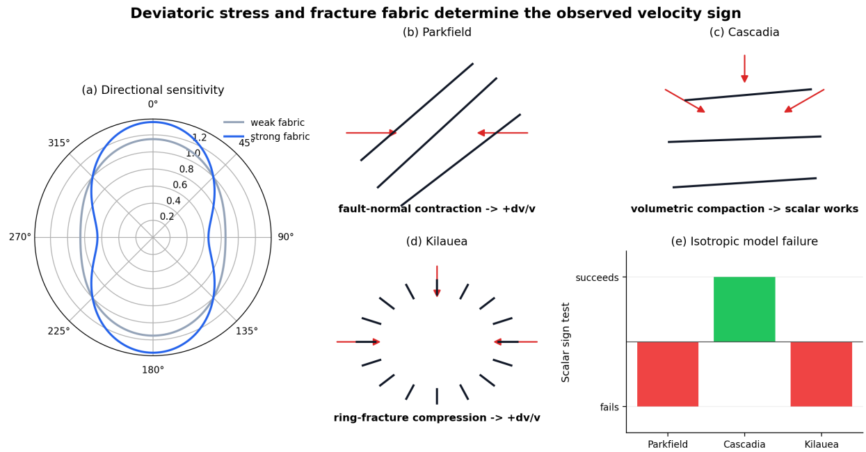
Figure 5: Deviatoric stress and fracture fabric determine the observed velocity sign. (a) Directional sensitivity increases with fracture fabric strength. (b–d) Parkfield, Cascadia, and Kīlauea select different stress/strain components because the dominant loading geometry and crack fabric differ. (e) Outcome of the scalar isotropic model by site (success at Cascadia; failure at Parkfield and Kīlauea).
