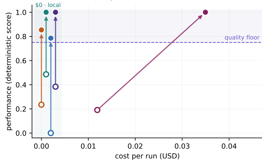
E2 · dv/v processing (parameter selection)
