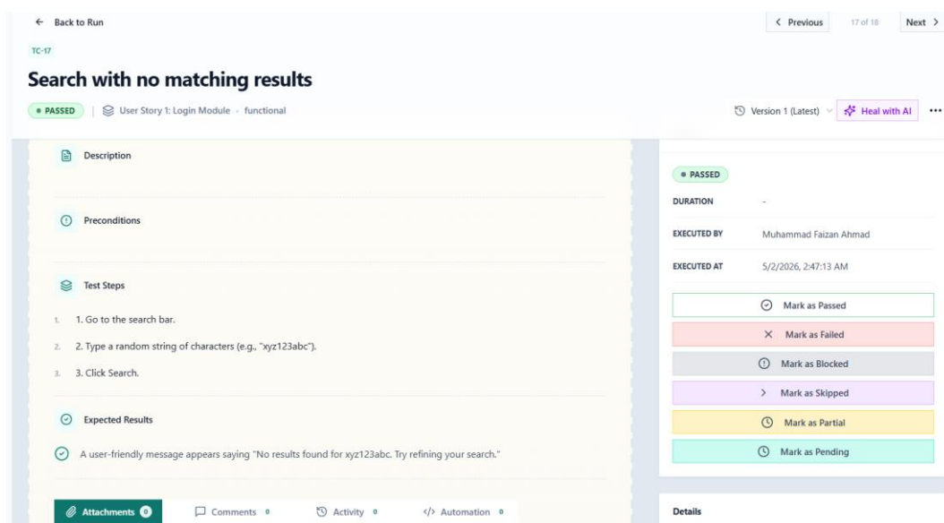
Fig 5.5 – TC-17 'Search with no matching results' – marked as PASSED
