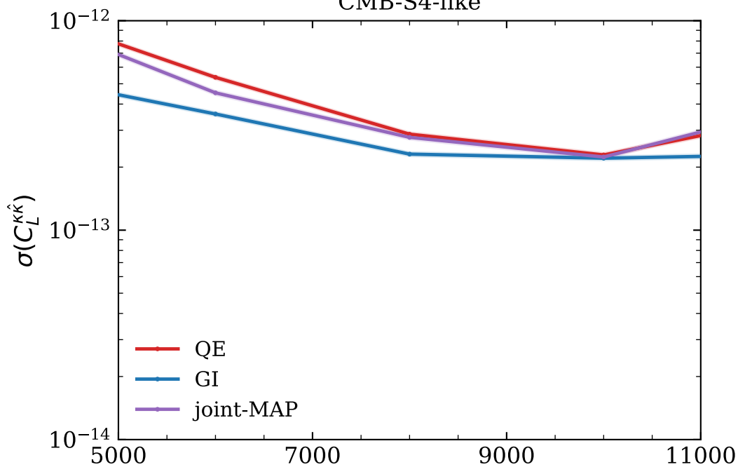
CMB-S4-like
