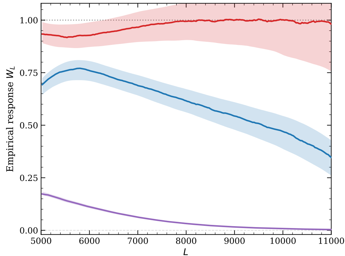
CMB-S4-like
