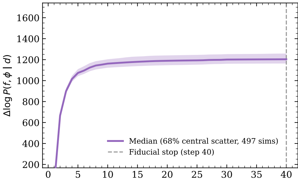
CMB-S4-like
